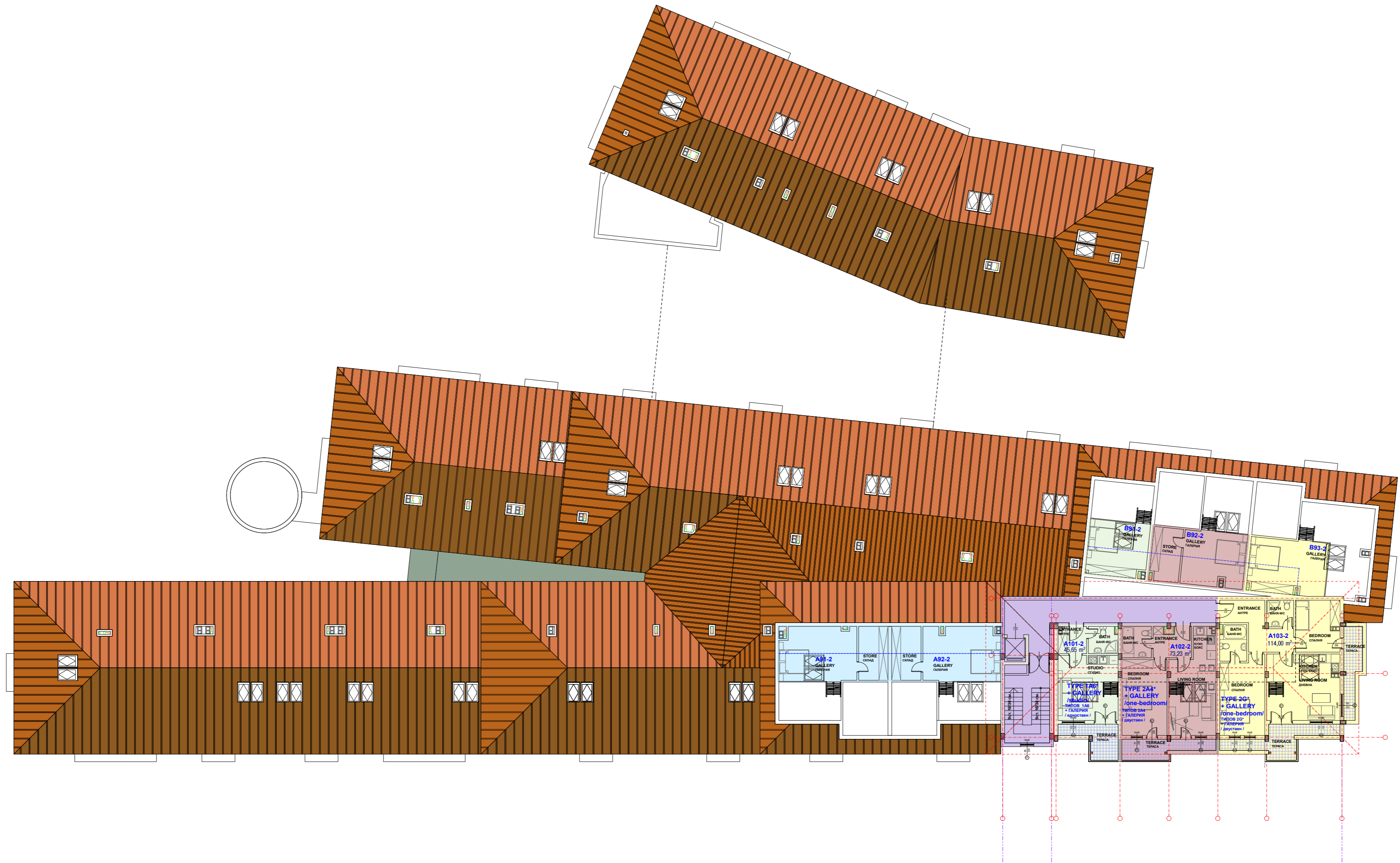
PLAN 10th STORY LEVEL +29,44 scale 1'200
